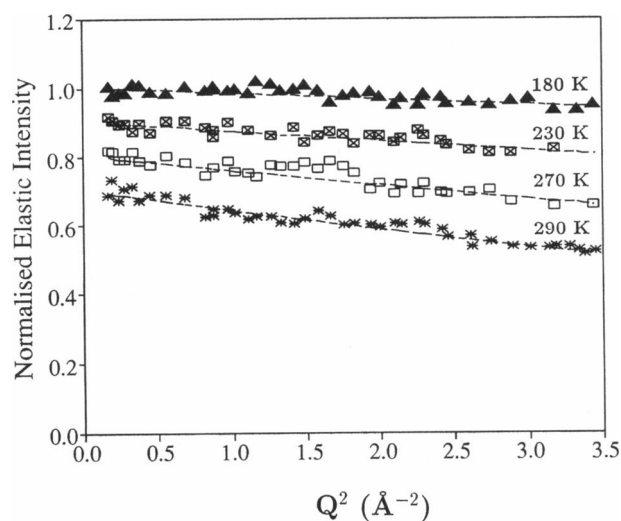
FIGURE 3 Normalized elastic intensity versus Q^2 for SOD at 0.25 hydration and for different temperatures: ( \Delta ) 180 K, ( \boxtimes ) 230 K, ( \square ) 270 K, and (*) 290 K. The linear fits are also indicated. The curves are shifted with respect to each other for better visibility.
