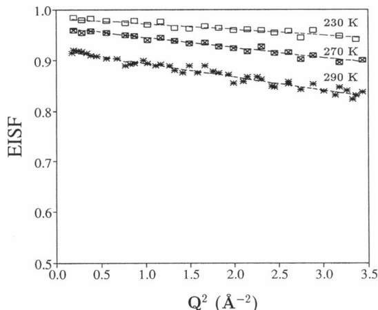
FIGURE 6 Elastic incoherent structure factor (EISF) versus Q^2 for a SOD sample at 0.25 hydration, and at different temperatures: ( \square ) 230 K, ( \times ) 270 K, and ( * ) 290 K.
